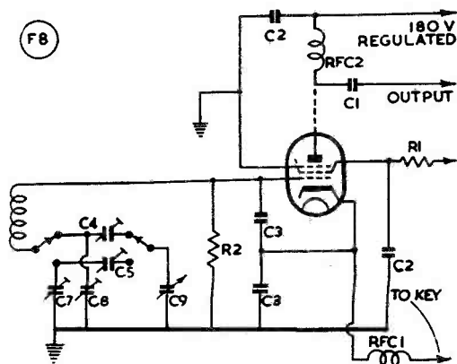
Fig. 2. A Clapp VFO with bandspread incorporated, as discussed in the text. The anode load, coupling and decoupling condensers are not mounted within the VFO box.
