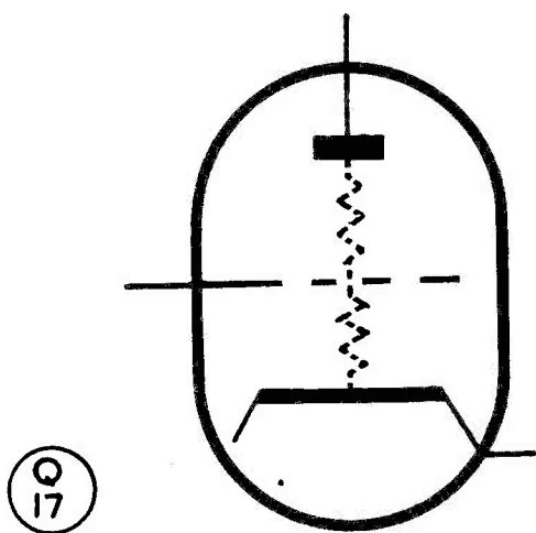
Fig. 1. The dotted resistors represent leakage paths between anode-grid and grid-cathode in a triode valve.
