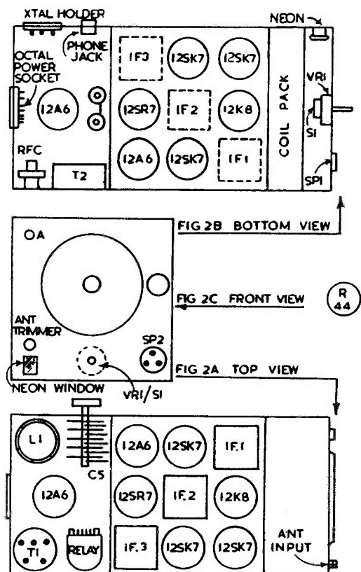
Fig. 2. Front, top and bottom view of the BC-455 showing main components and additional parts for carrying out the modifications suggested.
