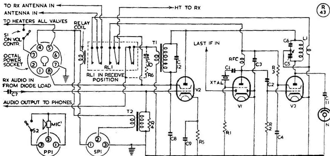
Fig. 1. Circuit of the transmitter section, showing receiver components common to both sections. All necessary values are given in the table.
