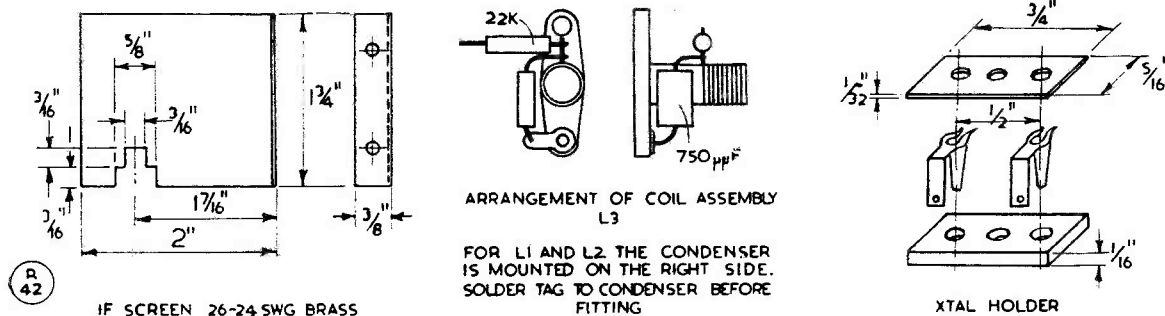
Fig. 3. Constructional details for screens and mountings for the G2DD 430 mc converter. Photographs of the model appeared on p. 749 of the February issue.
