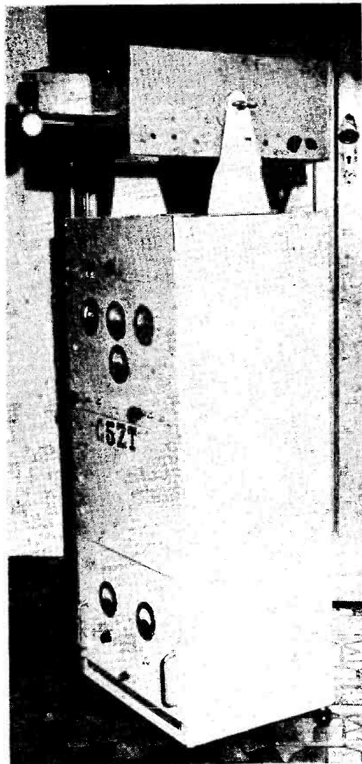
The complete TV transmitter now being operated on the 430 mc band by G5ZT/T of Plymouth, Devon. Pictures radiated by this equipment can be received on a standard BC TV receiver with the addition only of a simple converter and 430 mc aerial.
