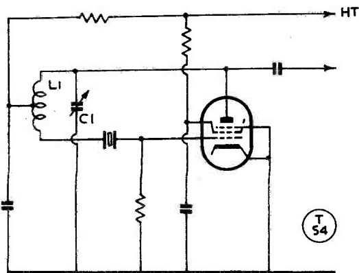
Fig. 1. The "Squier" overtone oscillator which is not suitable for even-harmonic working—see text.
