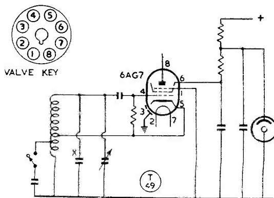
Fig. 2. The arrangement of Fig. 1 applied to another type of VFO. The basis of the idea is to be able to keep HT on the VFO, with the valve oscillating normally, but to prevent beating in the receiver on the operating channel. The effect is a high degree of VFO stability, as there is no HT switching, and therefore no change in valve temperatures and no variation in HT loading.
