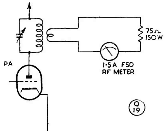
Fig. 3. Measurement of RF power output using a standard resistance, as explained in the text.
