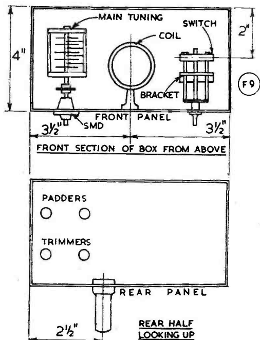
Fig. 3. Sketch showing general arrangement and layout of main components.
