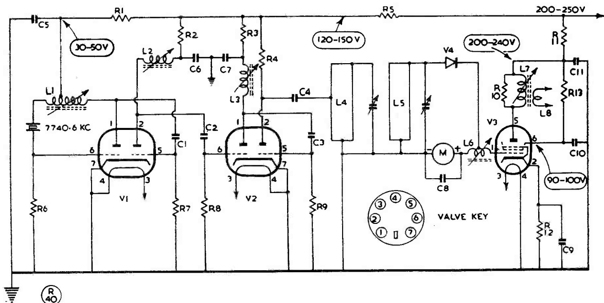
Fig. 1. Circuit of the Simplified 70-Centimetre Converter designed by G2DD. Elements marked L4, L5, are the brass strips for which dimensions are given in the coil table, the variable capacities across them being the air-spaced trimmers. The aerial coupling is arranged as described in the text.
