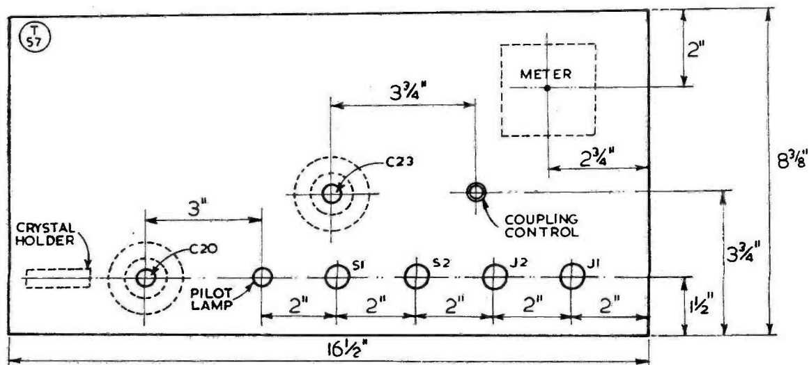
Fig. 4. Panel layout for the 10-metre Transmitter.
