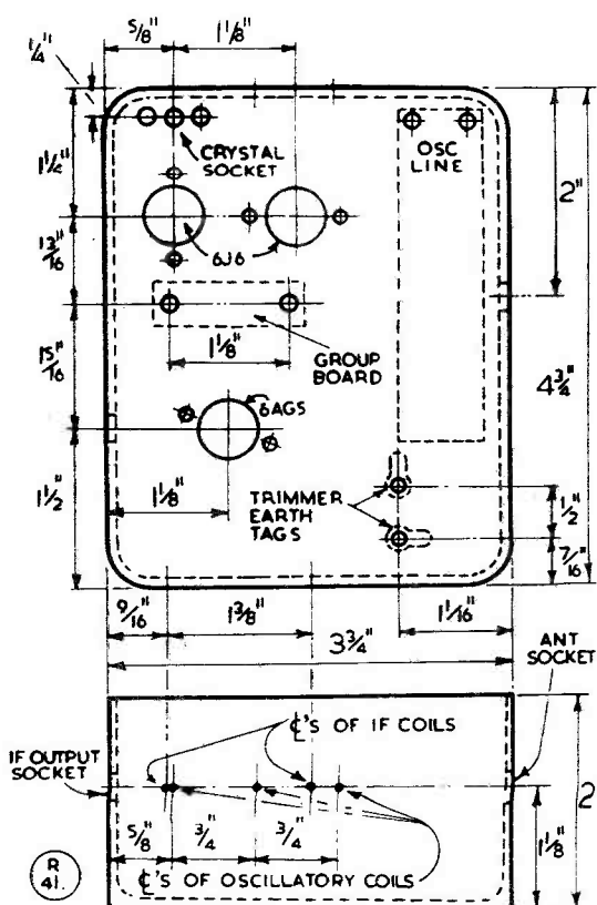
Fig. 2. Drilling detail and dimensions for mounting box for the G2DD Converter. It can be one of the standard Eddystone shapes.
