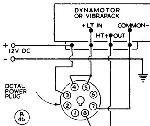
Fig. 3(B). The dynamotor or vibrator power supply connection. Note that pins 4, 5, are strapped.
