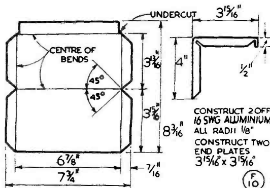
Fig. 4. Dimensions and details for construction of a suitable 7 x 4 x 4 ins. box for mounting the VFO. Material is 16g.
