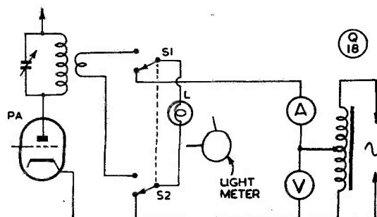
Fig. 2. Illustrating a comparison method of determining RF power output. It is sufficiently accurate for all practical purposes.
