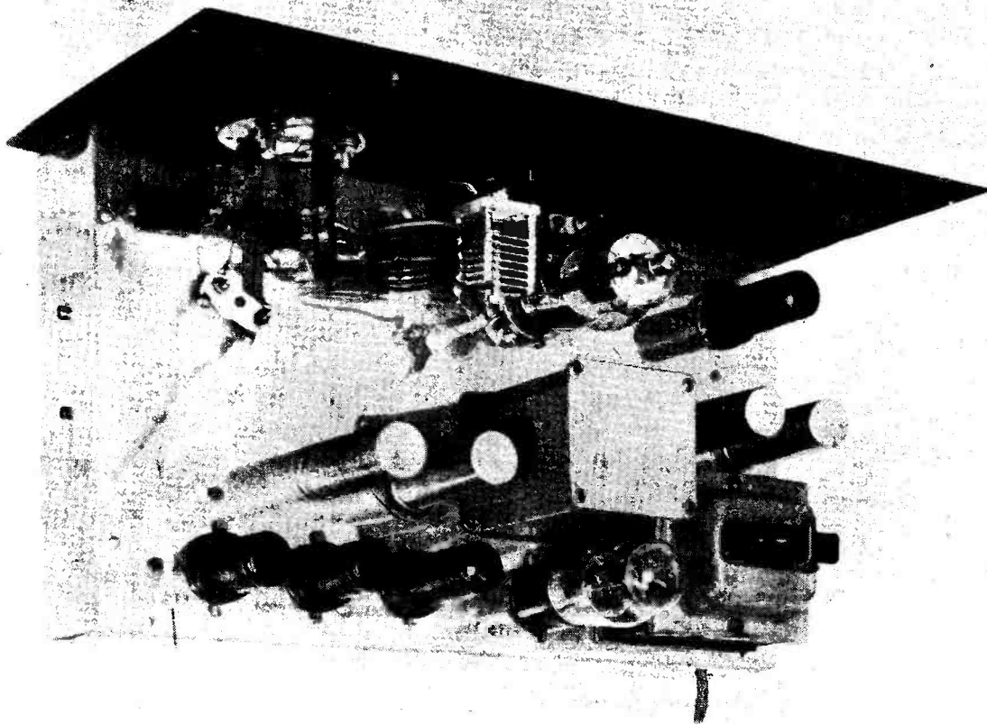
In this top view of the chassis of the Transmitter for Ten, note the positions of the neutralising condenser between PA valve and panel and the output coupling link. The general disposition of the parts will also be clear from this photograph.
