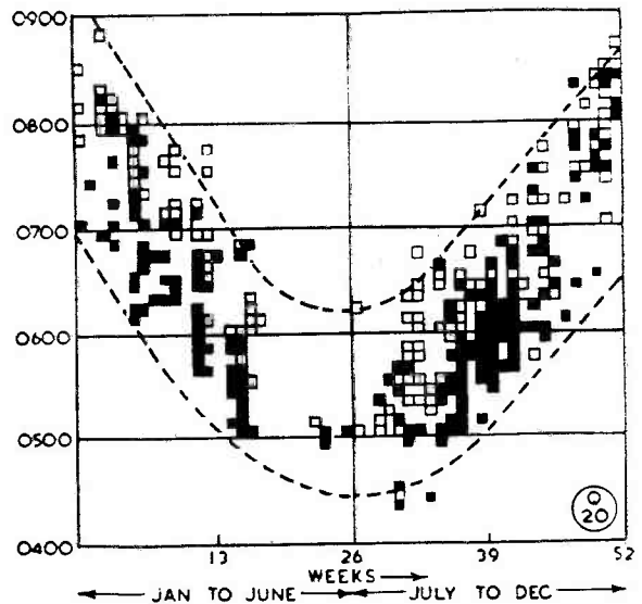
Fig. 1. Graphical representation of the volume of contacts obtained on the 40-metre band over the path Europe-New Zealand during the weeks of 1952, plotted against GMT.
