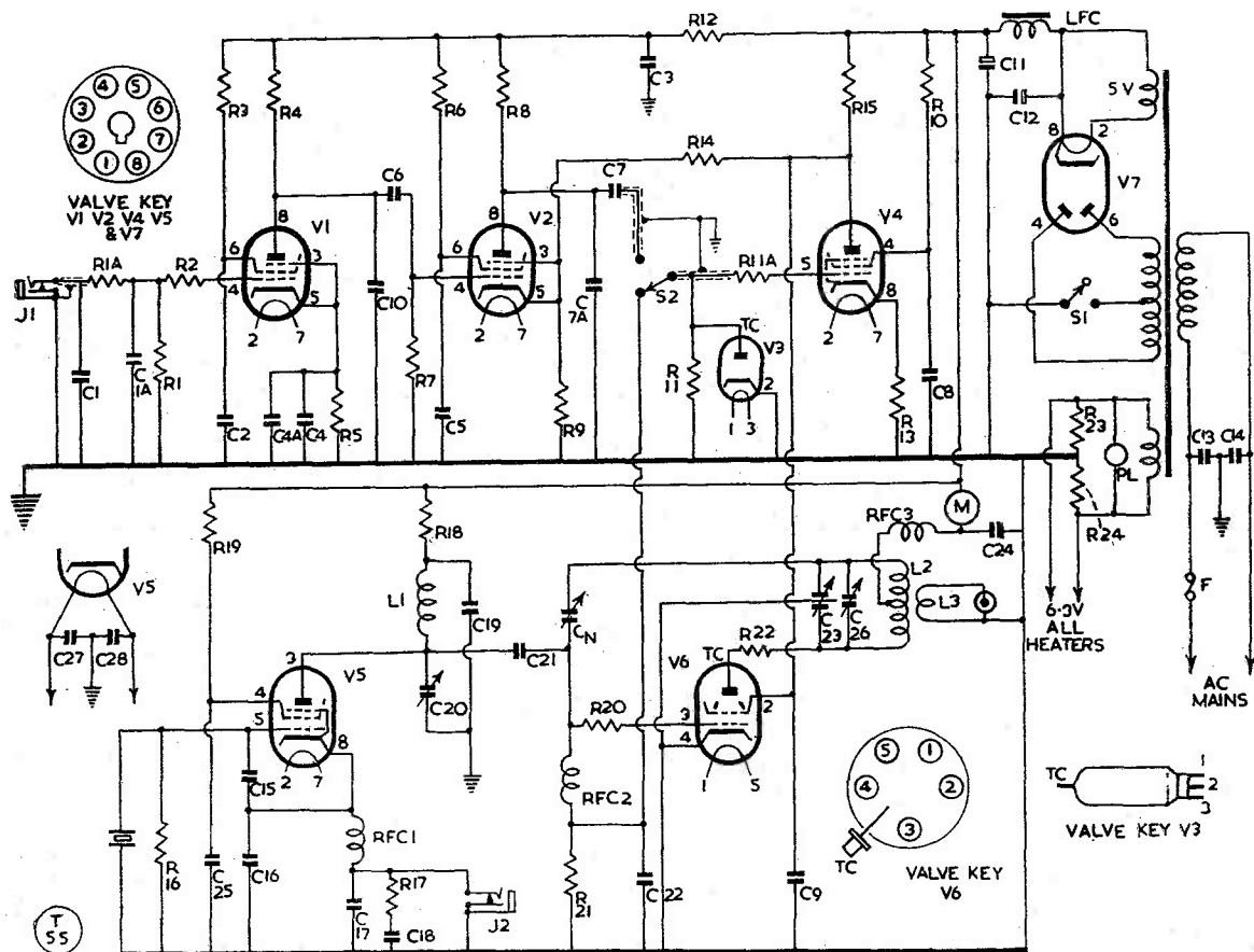
Fig. 2. Circuit diagram complete of the Transmitter for Ten. It is designed for crystal control and switch-on, switch-off operation. The only externals required are key (or microphone), aerial and AC power point.
