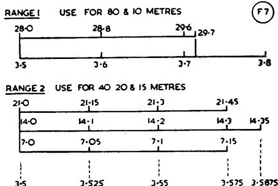
Fig. 1. Showing the two ranges for which the VFO can be set up and the bands to which they apply—see text.
