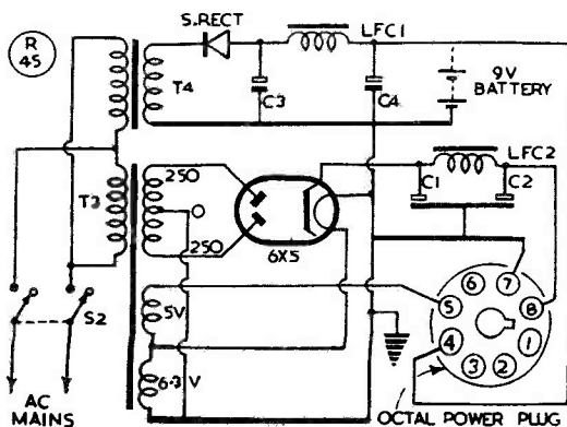
Fig. 3(A). Mains power unit, with LT windings connected in series to obtain 12v. heater supply. The 6X5 heater is tapped in at the junction.
