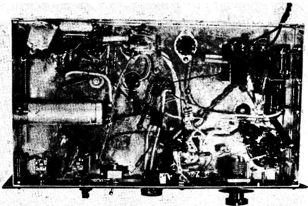
Layout beneath the chassis, showing wiring and placing of the major components.
