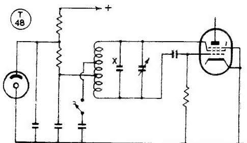
Fig. 1. A standard circuit is used for this VFO, the function of the switchable fixed condenser being to shift the frequency off the working channel under operating conditions.
